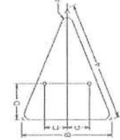
ISOSCELES TRIANGLE
