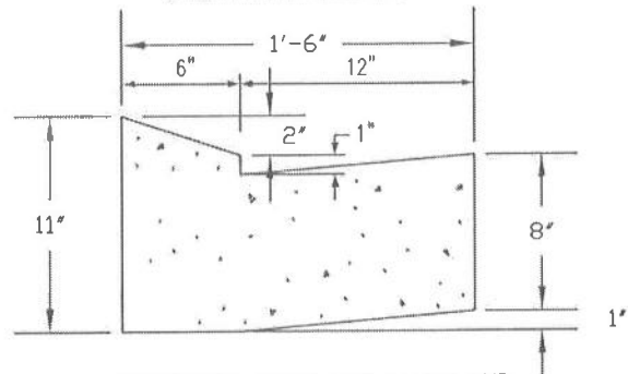
DEPRESSED CURB FOR LANES AND COMMERCIAL ESTABLISHMENTS
