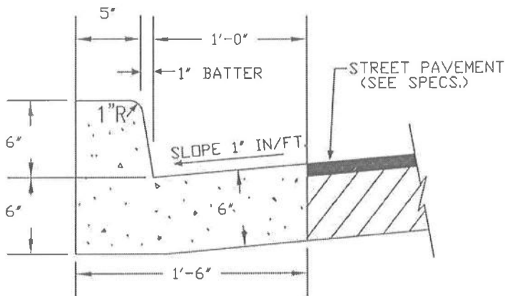
NORMAL GUTTER
