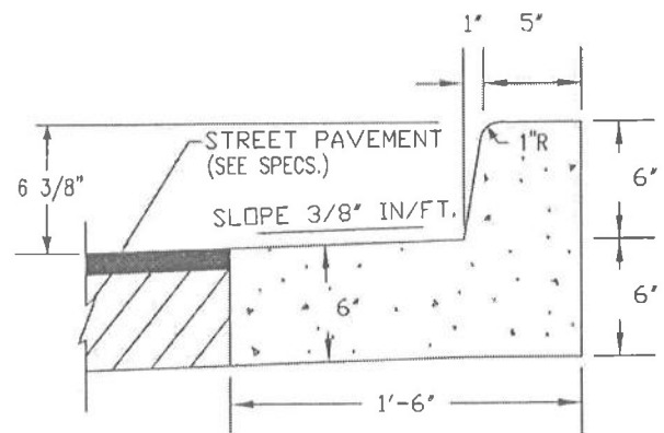
PITCHED GUTTER
