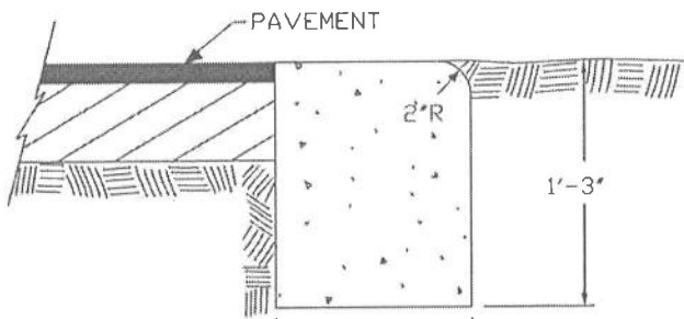
FLUSH HEADER CURB
