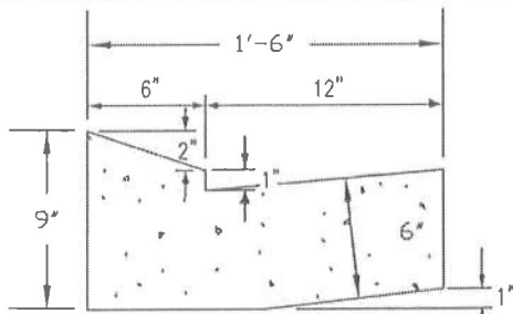
STANDARD DEPRESSED CURB AND GUTTER
