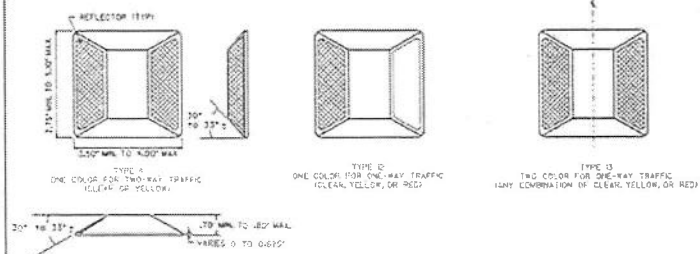
ALTERNATE RAISED REFLECTIVE MARKERS
