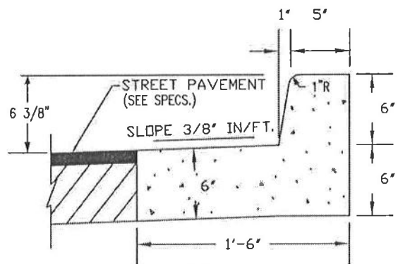
PITCHED GUTTER
