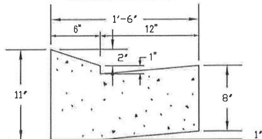
DEPRESSED CURB FOR LANES AND COMMERCIAL ESTABLISHMENTS
