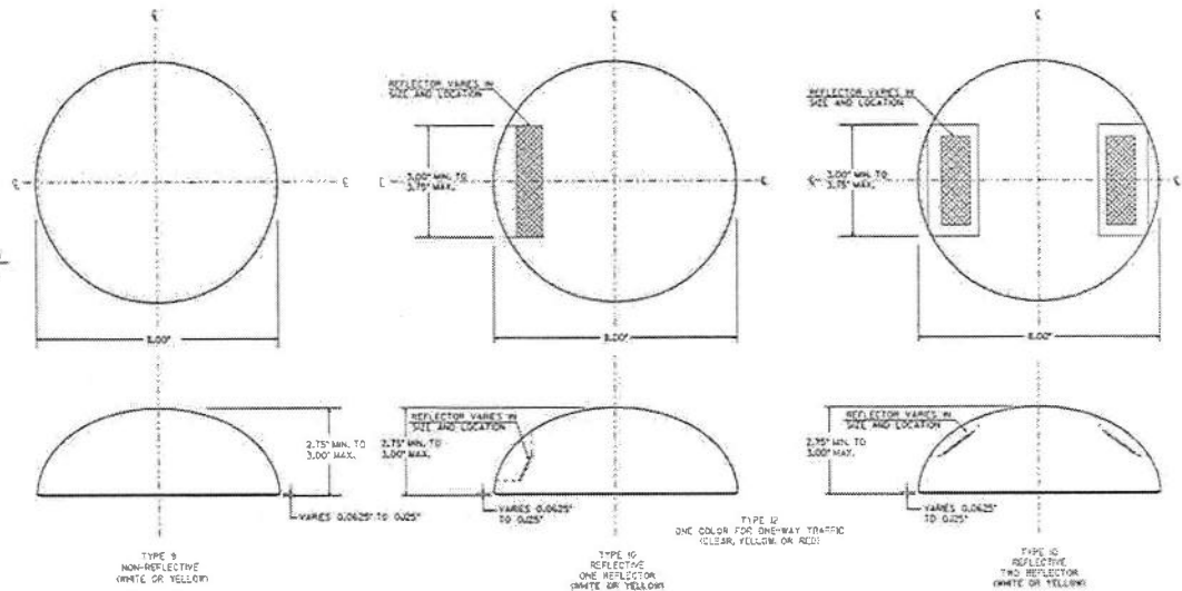
CERAMIC CHANNEL MARKER
