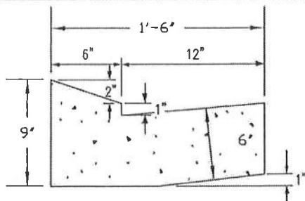
STANDARD DEPRESSED CURB AND GUTTER
