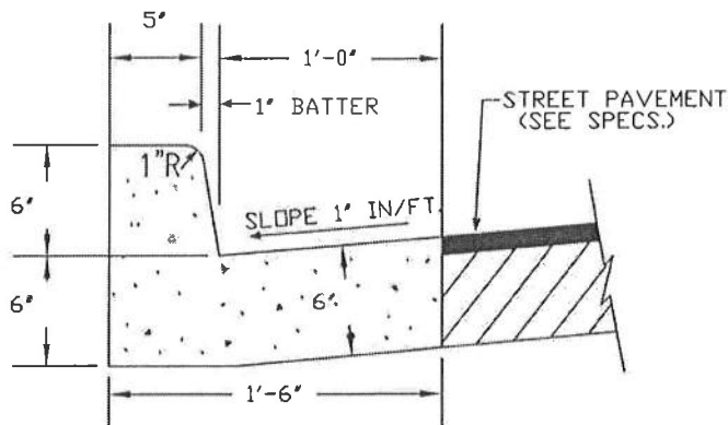
NORMAL GUTTER
