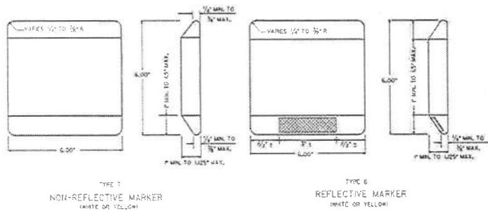
CERAMIC JIGGLE BAR MARKER
