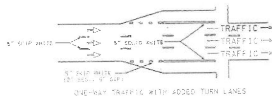
ONE-WAY TRAFFIC WITH ADDED TURN LANES
