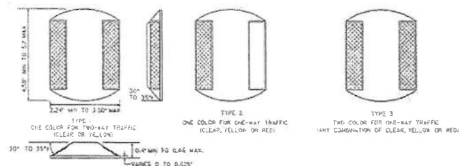
RAISED REFLECTIVE MARKERS
