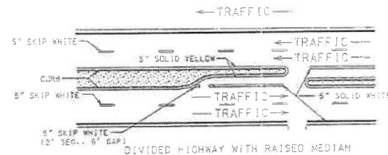
DIVIDED HIGHWAY WITH RAISED MEDIAN
