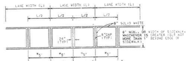
CROSSWALK DETAIL
