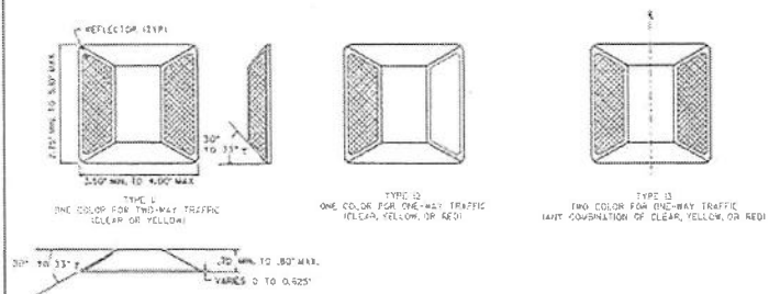
ALTERNATE RAISED REFLECTIVE MARKERS
