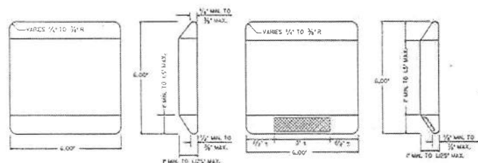
TYPE 7 NON-REFLECTIVE MARKER (WHITE OR YELLOW)
