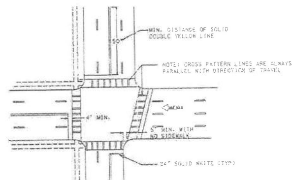
TYPICAL LOCATION OF CROSSWALKS AND STOP BARS
