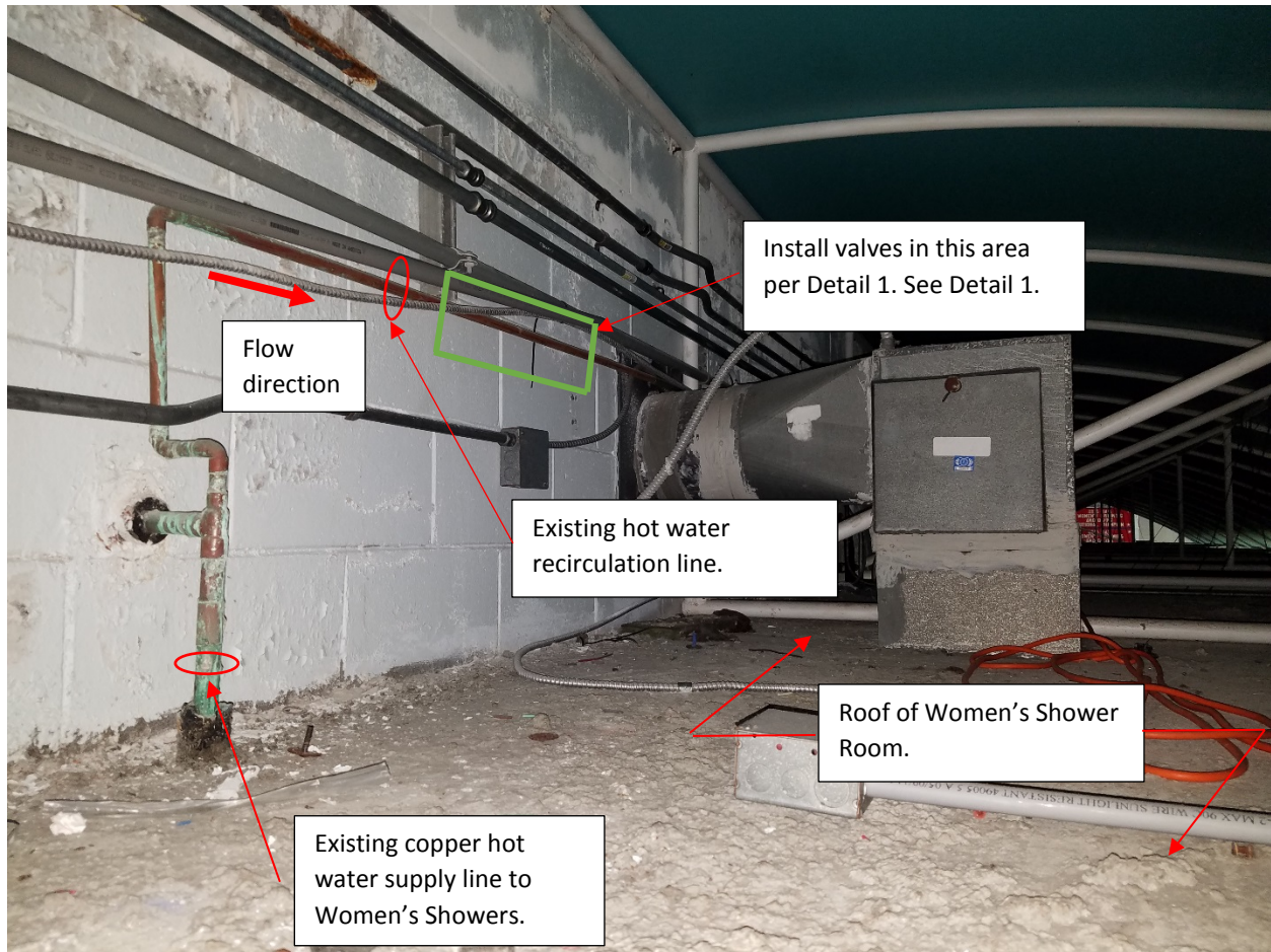
Women's Hot Water Recirculation Line Valve Installation
