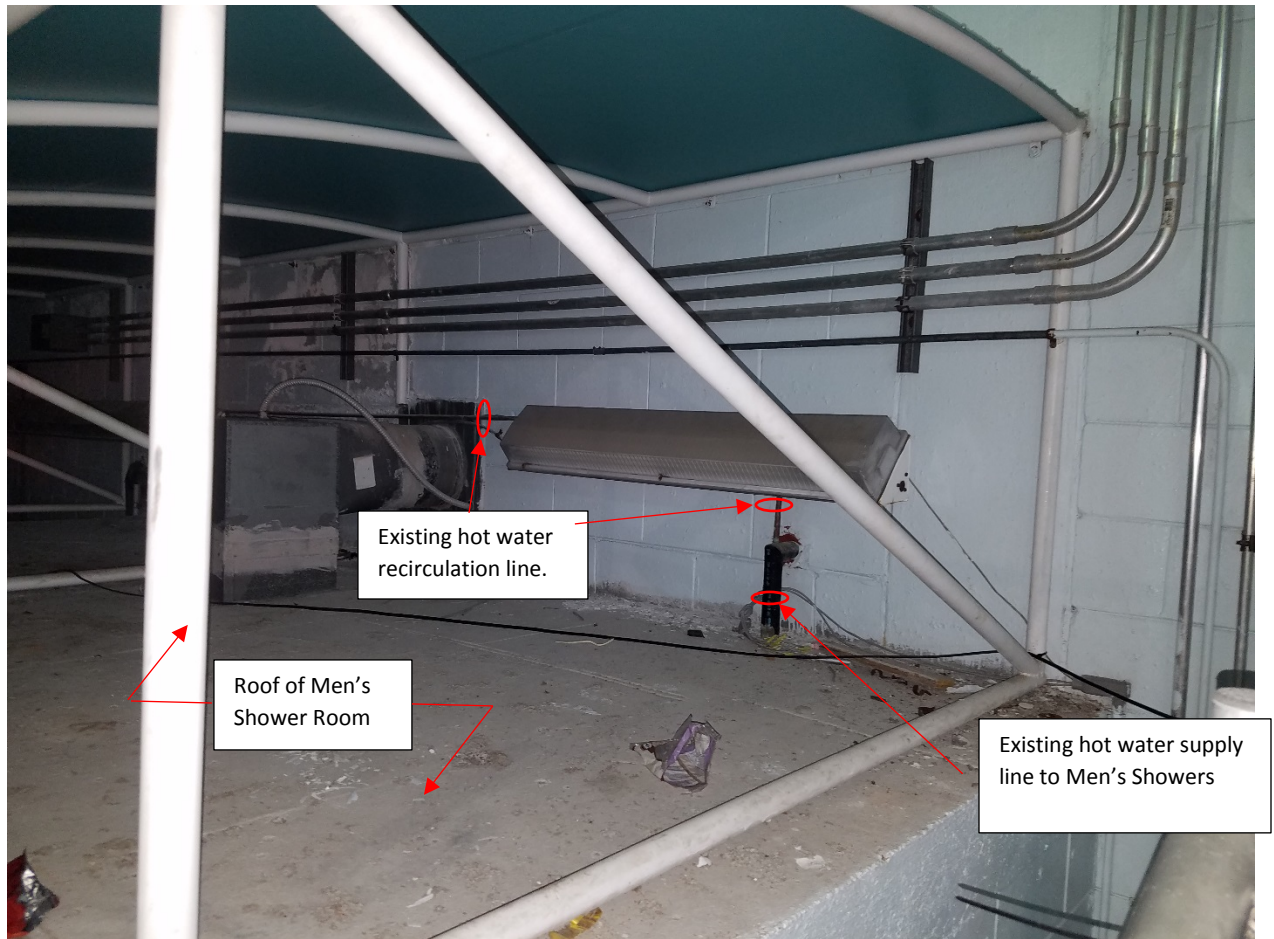
Men's Shower Room Roof
