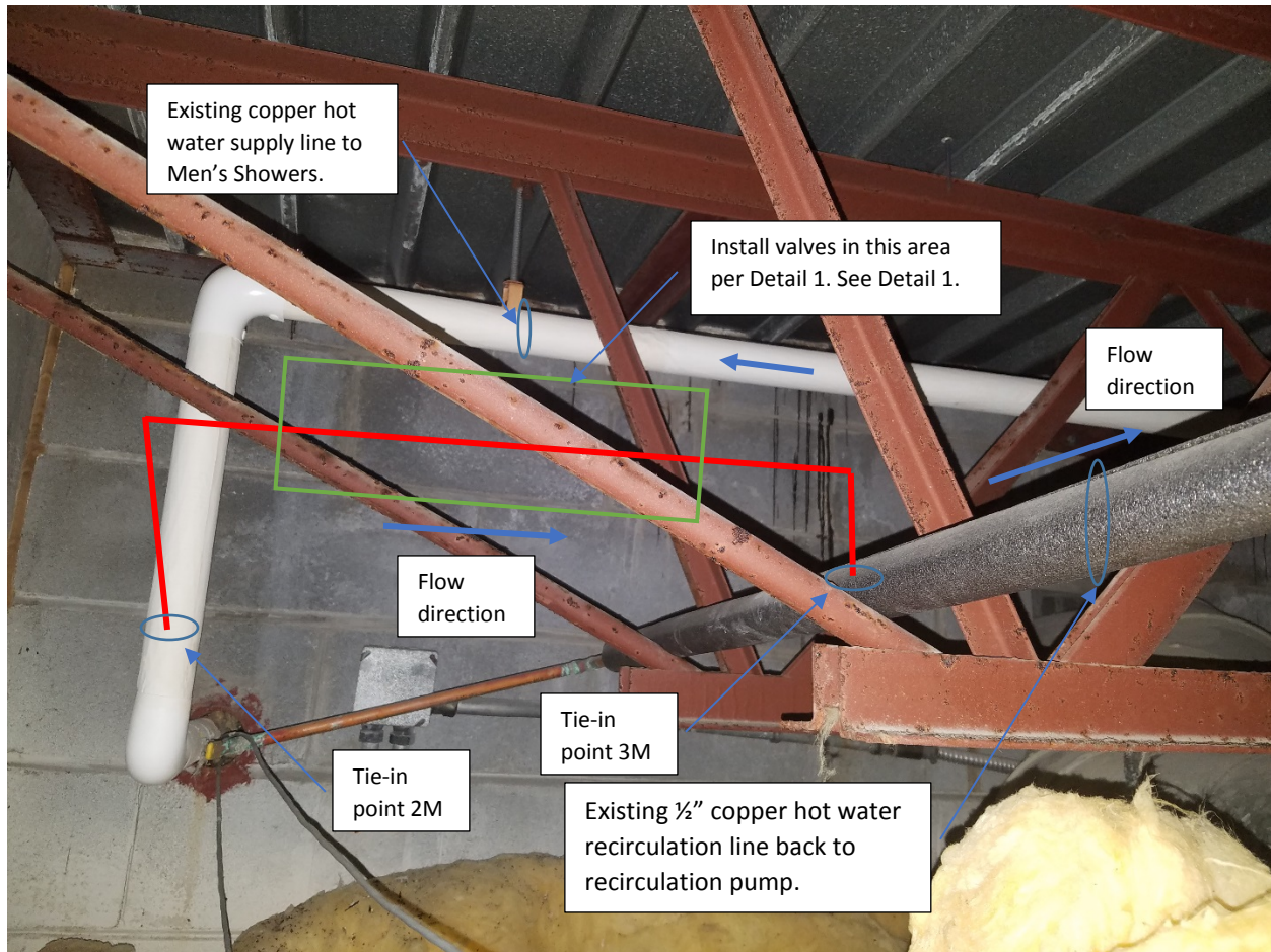
Men's Hot Water Recirculation Line Tie-in and Valve Installation
