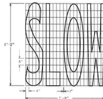
TYPE 5 AREA = 25.4 FT 2
