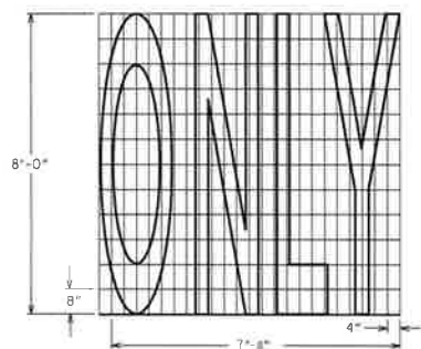
TYPE 1 AREA = 20.8 FT 2
