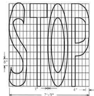
TYPE 2 AREA = 25.4 FT 2
