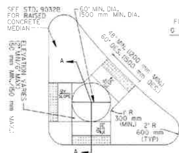
CONCRETE ISLAND WITH ELEVATED CUT THROUGH
