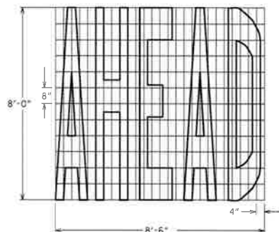
TYPE 4 AREA = 29.1 FT 2
