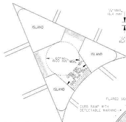
CONCRETE ISLAND WITH ELEVATED CUT THROUGH
