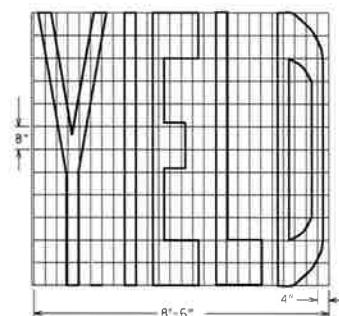
TYPE 15 AREA = 25.4 FT 2
